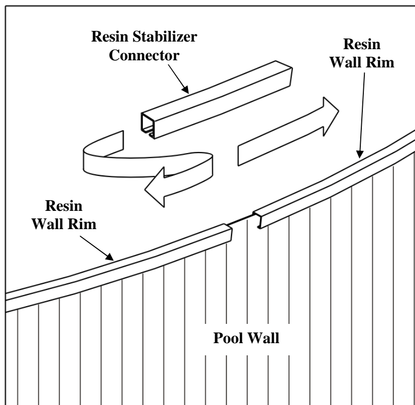
Resin Stabilizer Connector Installation
